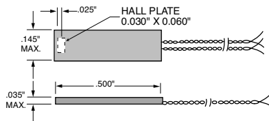
Model BH-207 High Resolution Tangential
