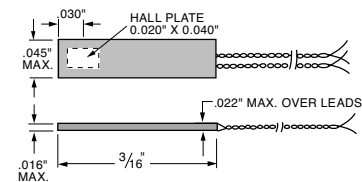
Model BH-209 Ultra-Mini Transverse
