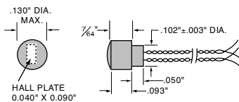
Model BH-202 Small Axial
