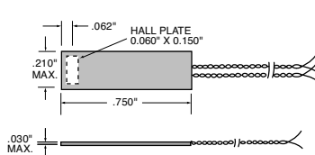
Model BH-206 High Sensitivity Low Cost Transverse
