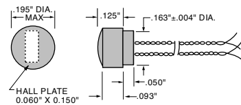
Model BH-203 General-Purpose Axial
