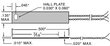
Model BH-201 Ultra-Thin Transverse
