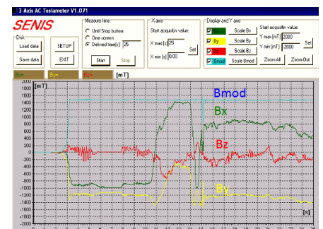
Figure 1. 3-Axis magnetic field Teslameter 3MH3A with fully integrated Hall Probe
