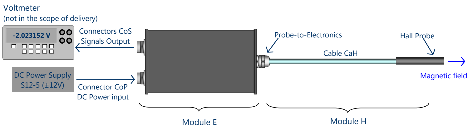
Figure 1. Typical measurement setup with a SENIS magnetic-field-to-voltage transducer with integrated Hall Probe (Module H) and Electronic (Module E)
